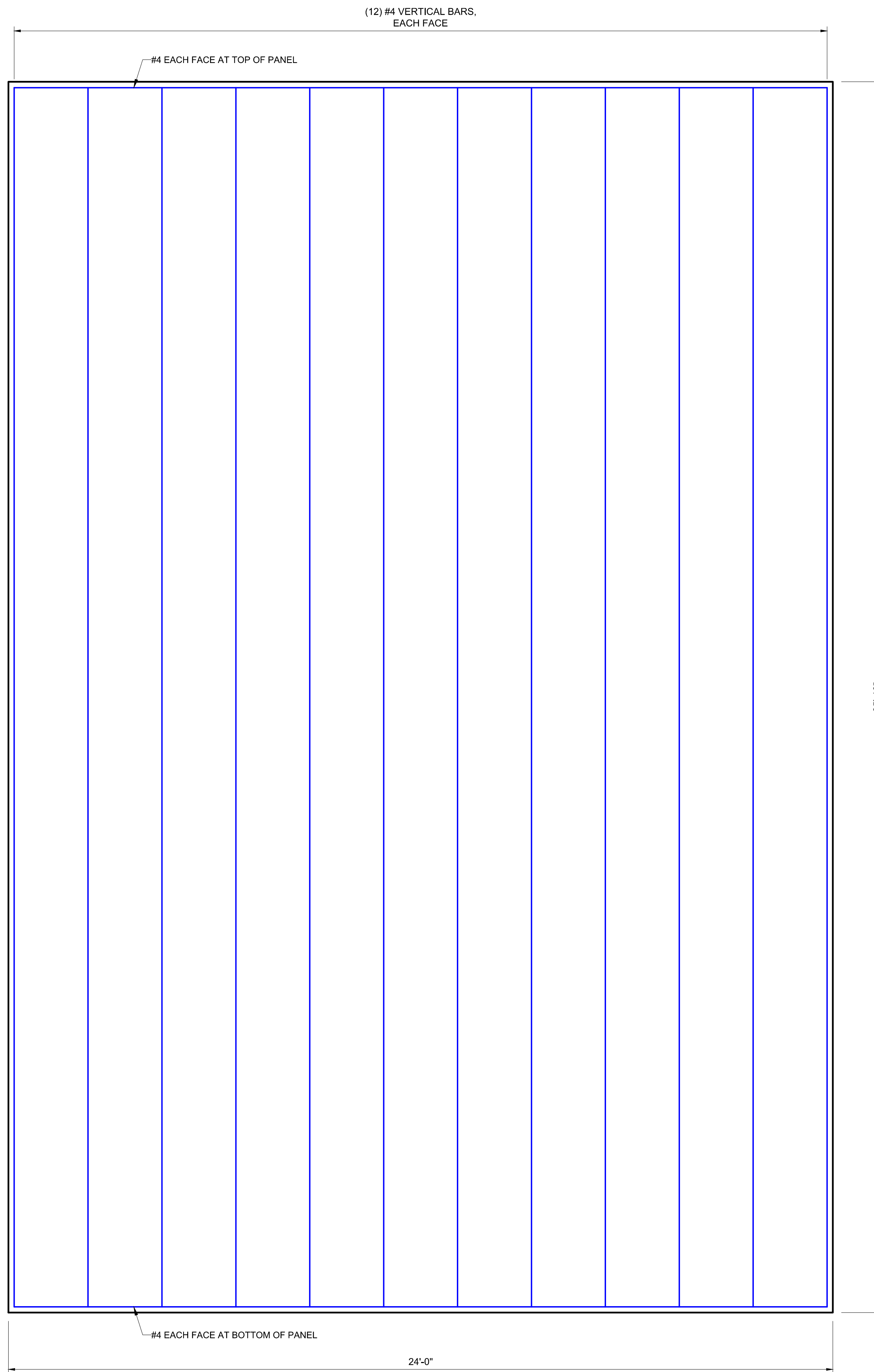
TIPS REINFORCING 1/2" = 1'-0"
