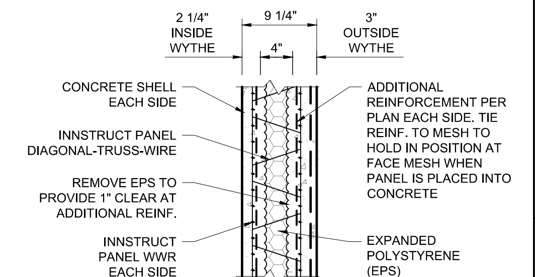
TYPICAL INNSTRUCT PANEL SCALE: NTS
